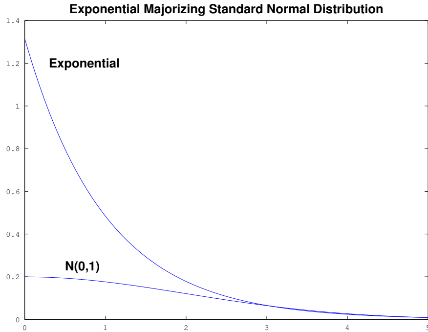
Figure 10.8: A graph showing the exponential pdf majorizing the standard normal pdf.
