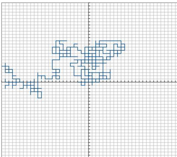
Figure 10.11: A random walk generated by Listing 10.4.
