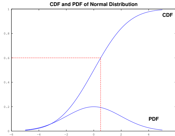
Figure 10.6: A probability density function (pdf) and its cumulative distribution function (CDF), in this case a normal distribution n(x; \mu, \sigma) , and the inverse mapping from the interval [0, 1] to a sample from n(x; \mu, \sigma) .
