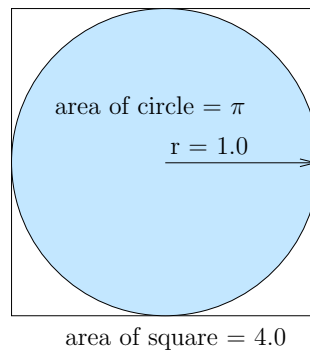
Figure 10.1: A circle in a square whose side equals its diameter. If the diameter is 2, then the square has area 4 and the circle has area \pi . The ratio of the circle's area to the square's is \pi/4 .
