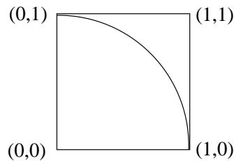
Figure 10.2: A quarter circle of unit radius in a square of unit width.
