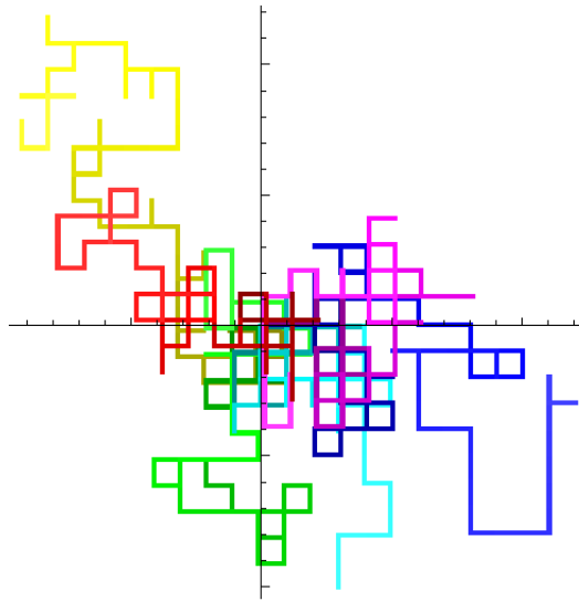
Figure 10.10: A sequence of random walks from the origin of a 2D grid.
