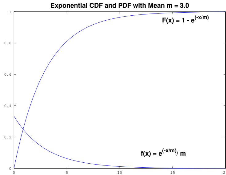
Figure 10.7: Graph of the exponential distribution pdf and cdf with mean 3.0.
