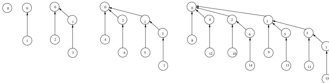
(b) This is the same representation of the binomial tree but the nodes have been relabeled to correspond to the reduction algorithm described in the text. The node labels do not correspond in a natural way to how the trees can grow recursively, but they do correspond to how processes can communicate in a parallel reduction.
