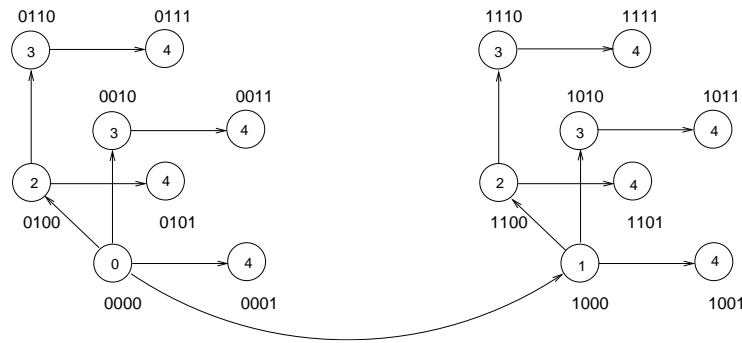
Figure 3.26: Propagation of node 0's data item along a reverse binomial tree rooted at 0. The numbers inside the nodes indicate in which iteration that node first gets node 0's data item. These numbers correspond to the bit position that was used in that step, with 0 being the leftmost bit.
