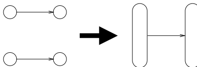
Figure 3.10: Agglomerating to reduce message transmissions. By combining the two tasks that send, and the two that receive, into a single task each, the number of transmissions is reduced, decreasing message latency.
